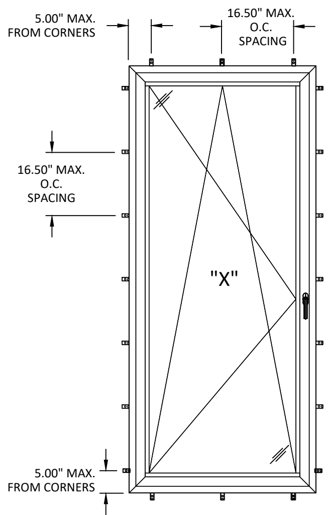
ANCHOR LAYOUT STRAP INSTALLATION
