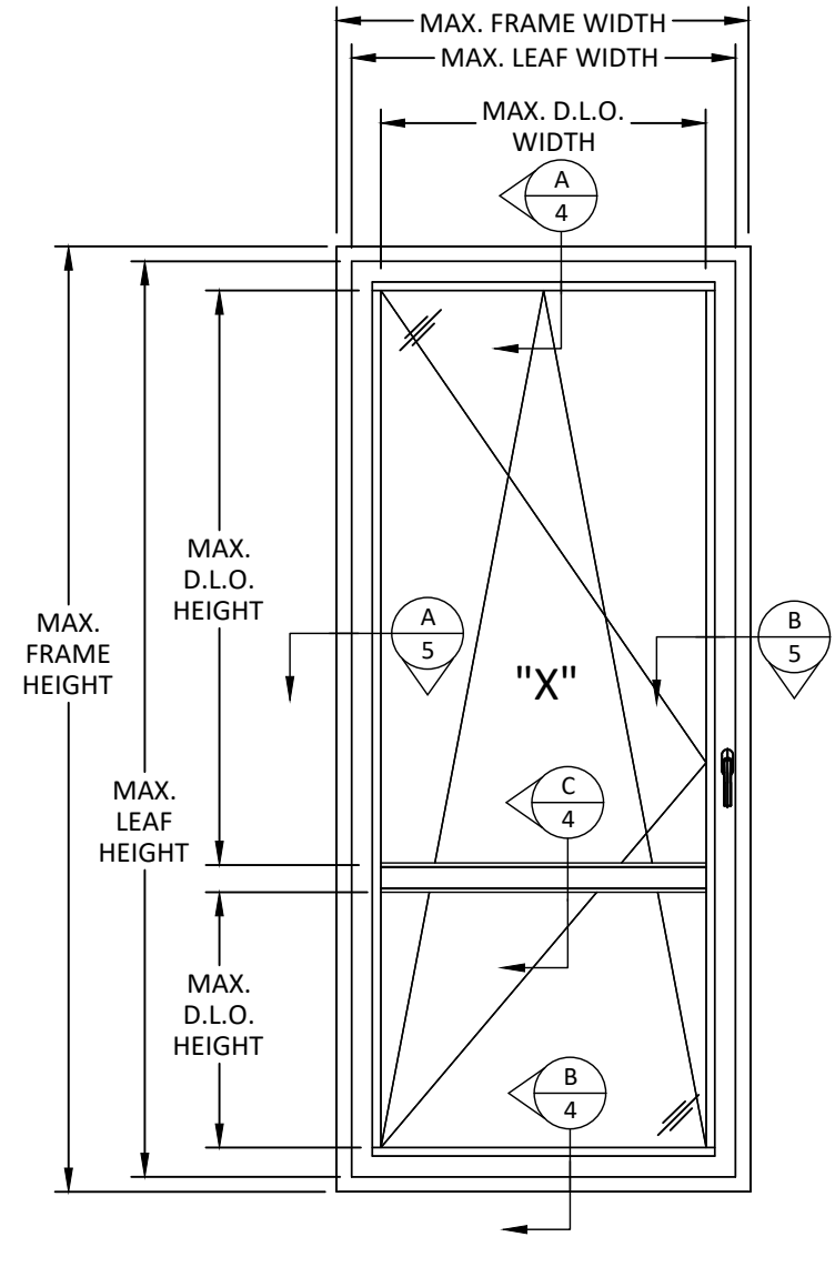
ELEVATIONS
