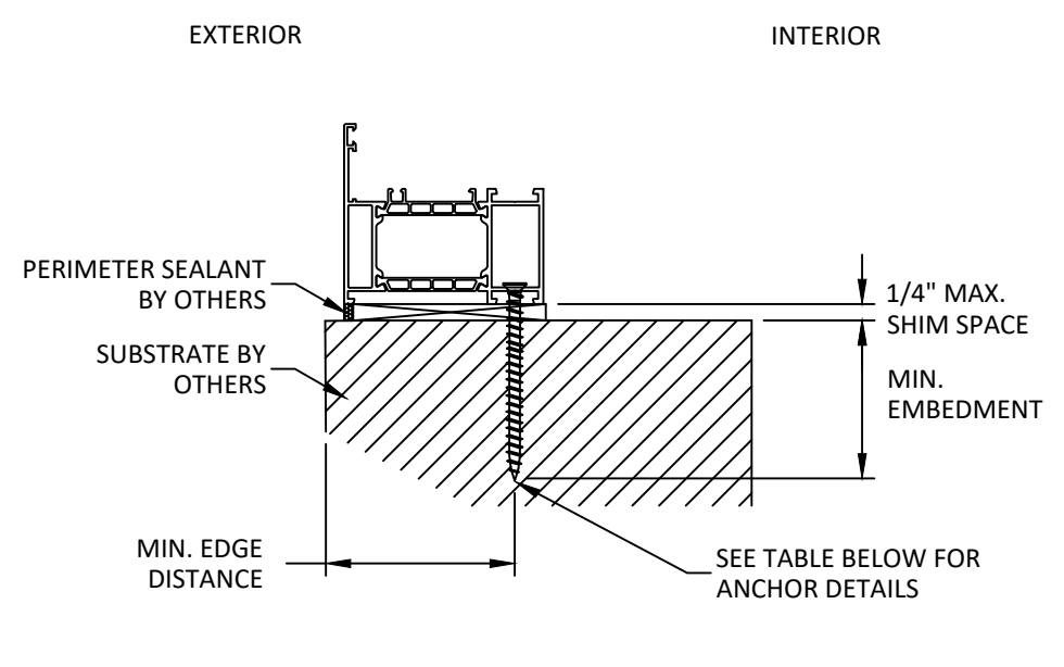
B 6 VERTICAL SECTION THROUGH FRAME INSTALLATION
